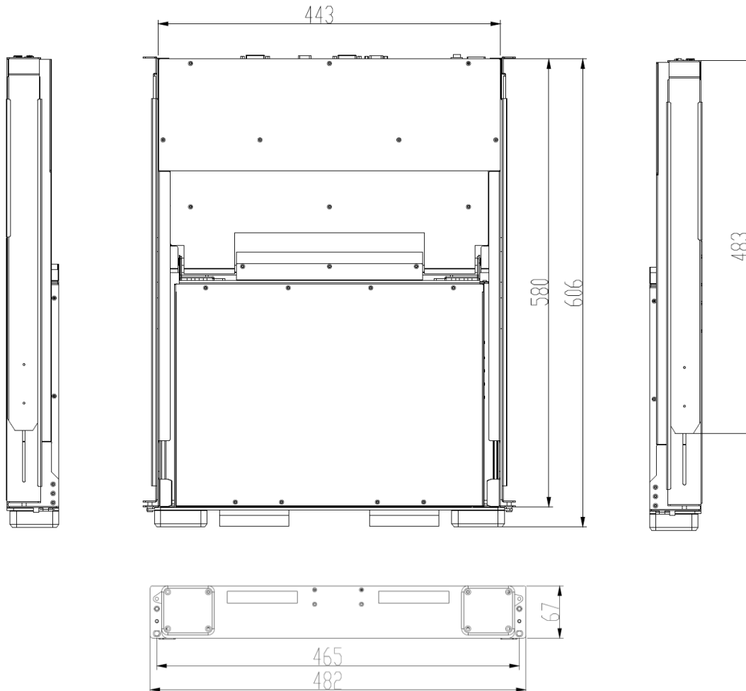
Rear of KVMD-1701W-D2
